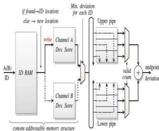
Figure 3 Architecture Of Custom Flex-Ray Communication Controller
