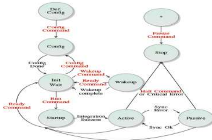
Figure 2 Flex-Ray Cc Modes
