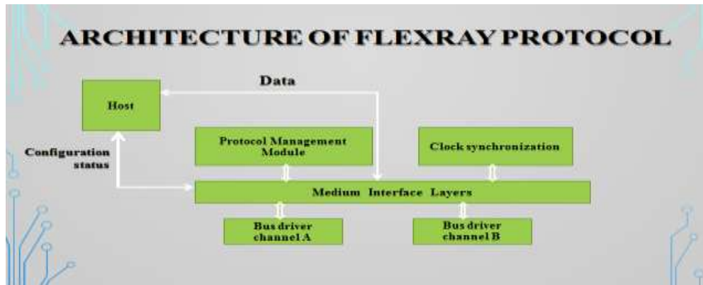
Figure1 Architecture Of FlexRay Protocol
